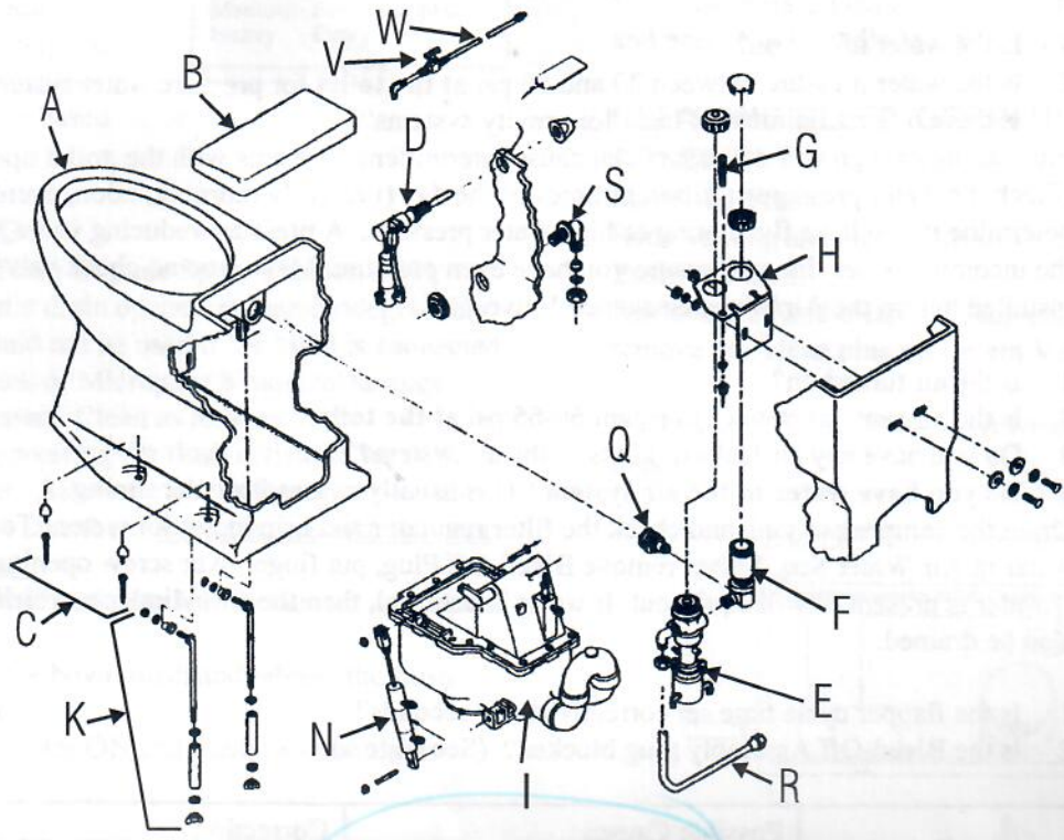
Integral Valve Layout
